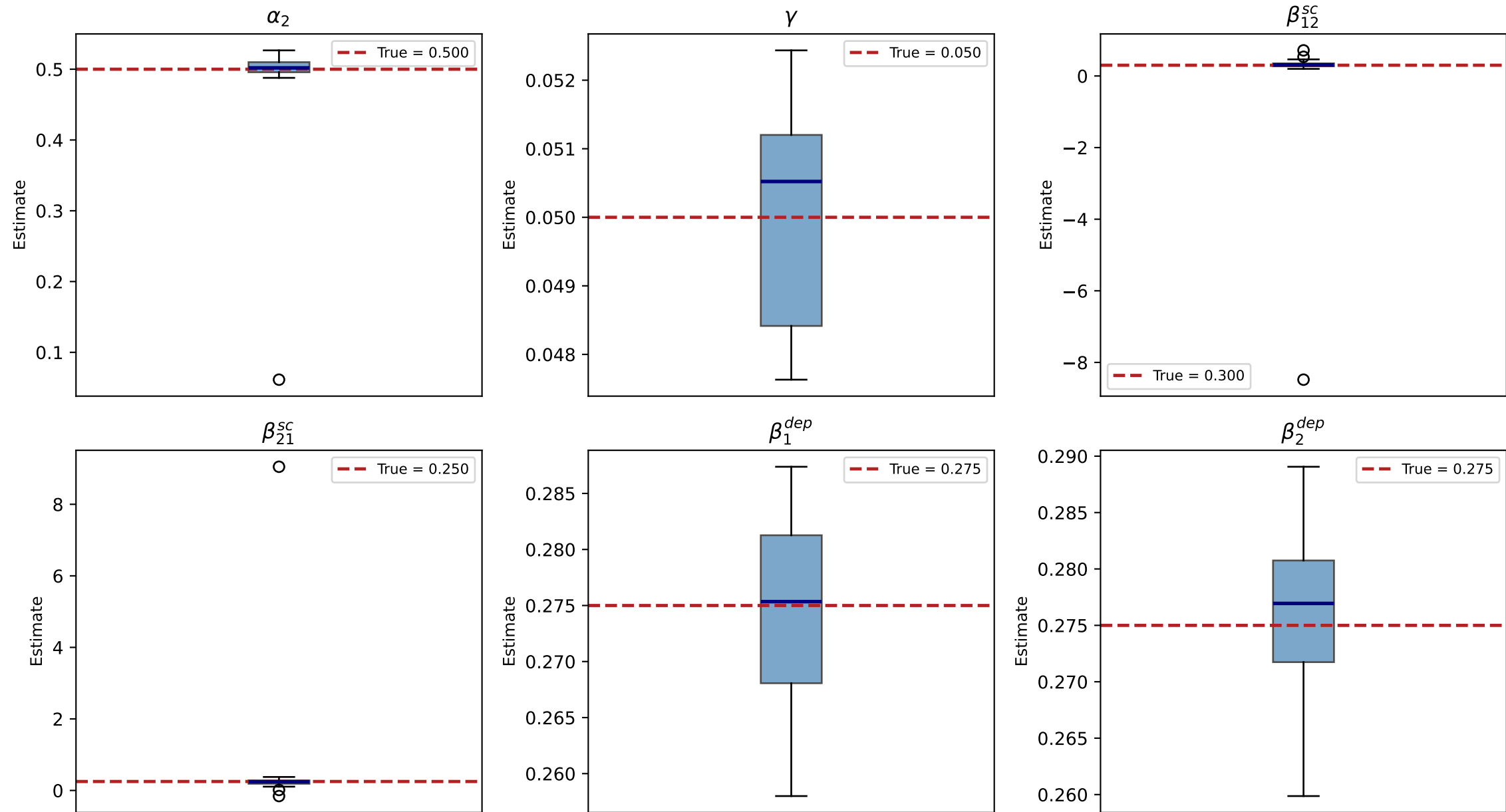
NFXP Monte Carlo: original model ( \beta^{dep} brand-specific) (reps=20, N=2000, T=52)
